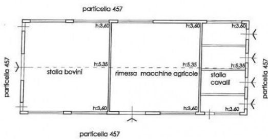
PIANO TERRENO
