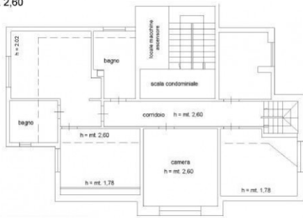
PIANO QUINTO IH = MT. 2,60
